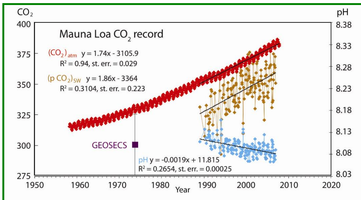
Figure 5.5 Time series of atmospheric \text{CO}_2 at Mauna Loa (in parts per million volume, ppmv) (red), surface ocean pH (cyan), and seawater p\text{CO}_2 ( \mu\text{atm} ) (tan) at Ocean Station ALOHA in the subtropical North Pacific Ocean (from Doney et al., 2009). Note that the increase in oceanic \text{CO}_2 over the past 17 years is consistent with the atmospheric increase within the statistical limits of the measurements. Geochemical Ocean Section Study (GEOSECS) data are from a station near Station ALOHA collected in 1973 (data from Takahashi et al., 1980).
